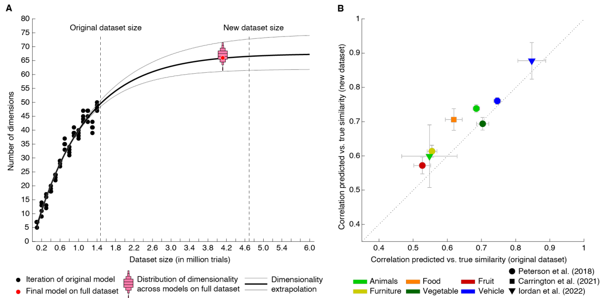
Fig. 3. Behavioral similarity dataset. A. How much data is required to capture the core representational dimensions underlying human similarity judgments? Based on the original dataset of 1.46 million triplets 30 , it was predicted that around 4.5-5 million triplets would be required for the curve to saturate. Indeed, for the full dataset, the dimensionality was found to be 66, in line with the extrapolation. Red bars indicate histograms for dimensionality across several random model initializations, while the final model was chosen to be the most stable among this set. B. Within-category pairwise similarity ratings were predicted better for diverse datasets using the new, larger dataset of 4.70 million triplets (4.10 million training samples), indicating that this dataset contains more fine-grained similarity information. Error bars reflect standard errors of the mean.
