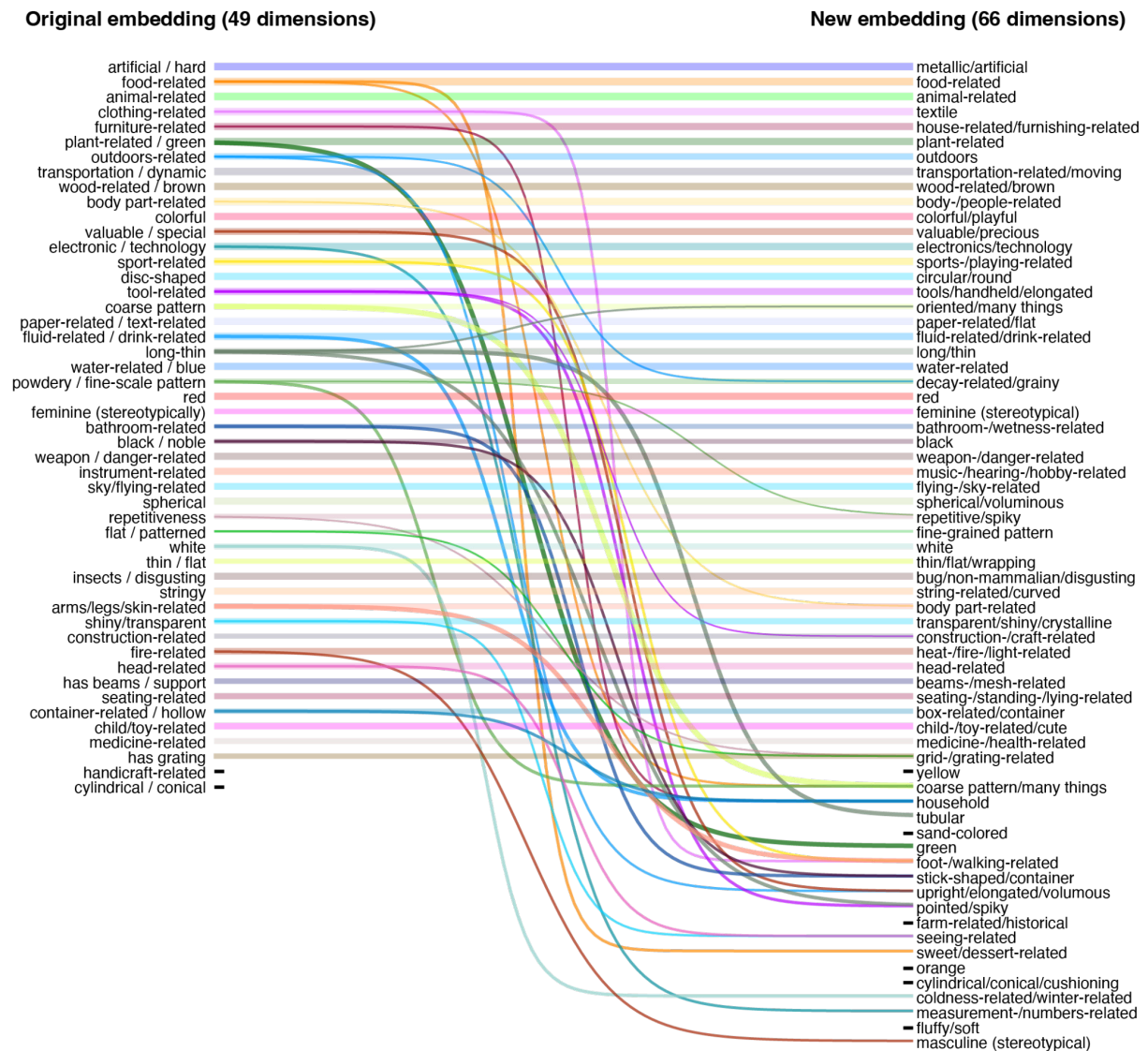
Supplementary Fig. 7. Changes in embedding dimensions between original embedding (49 dimensions) and the new embedding (66 dimensions) based on the full dataset. Lines correspond to Pearson correlations between old and new dimensions, only showing cases with r > 0.3 for dimensions that already have a strong pairing (e.g. “artificial/hard” with “metallic/artificial”) and r > 0.3 for dimensions without a strong pairing (after correcting for baseline cross-correlation between the original 49 dimensions). These cutoffs were chosen arbitrarily to provide a trade-off between maximizing the information contained in this figure while still effectively visualizing changes in dimensions. 46 out of 49 original dimensions showed strong correlations with new dimensions (all r > 0.63 ), demonstrating that the original embedding was reproduced well. In addition, several dimensions were split up, either revealing more fine-grained distinctions (e.g. “sweet/dessert” rather than “food”), disentangling dimensions further (e.g. “plant-related/green” to separate dimensions for “plant-related” and “green”), or sometimes remixing them (e.g. “tool-related” and “long/thin” led to “pointed/spiky”). Finally, there were a number of dimensions that previously had not been found and also showed no strong relationship to previous dimensions (e.g. “fluffy/soft”).
