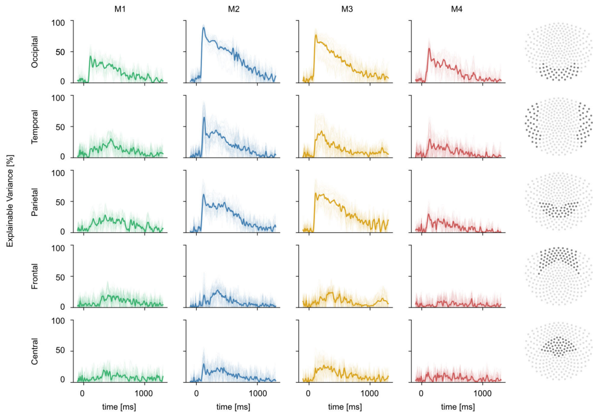
Supplementary Fig. 4. MEG noise ceilings for all sensors. Every column shows the noise ceiling for a given participant. The last column highlights which sensors were considered for each sensor group (row). Noise ceilings were calculated for each sensor (thin lines) and averaged across sensors in a given sensor group (thick line).
