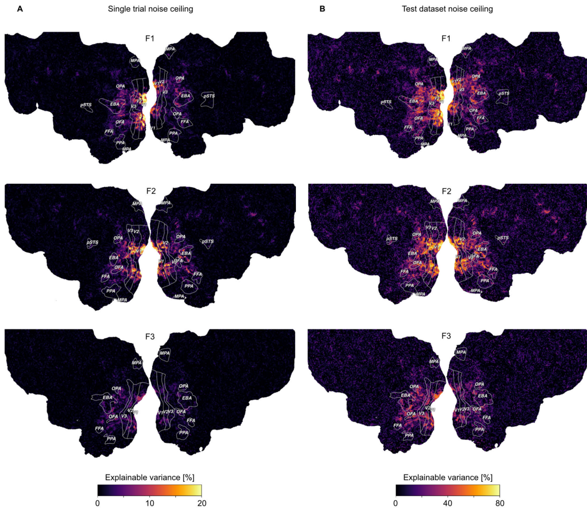
Supplementary Fig. 5. fMRI voxel-wise noise ceilings per participant projected onto the flattened cortical surface. A. The noise ceiling estimate on the level of single trial responses. B. Noise ceiling estimate in the test dataset where responses from 12 trial repetitions can be averaged. Note that the range of noise ceiling values represented by the color map is higher for the test dataset (0-80%) compared to the single trial responses (0-20%).
