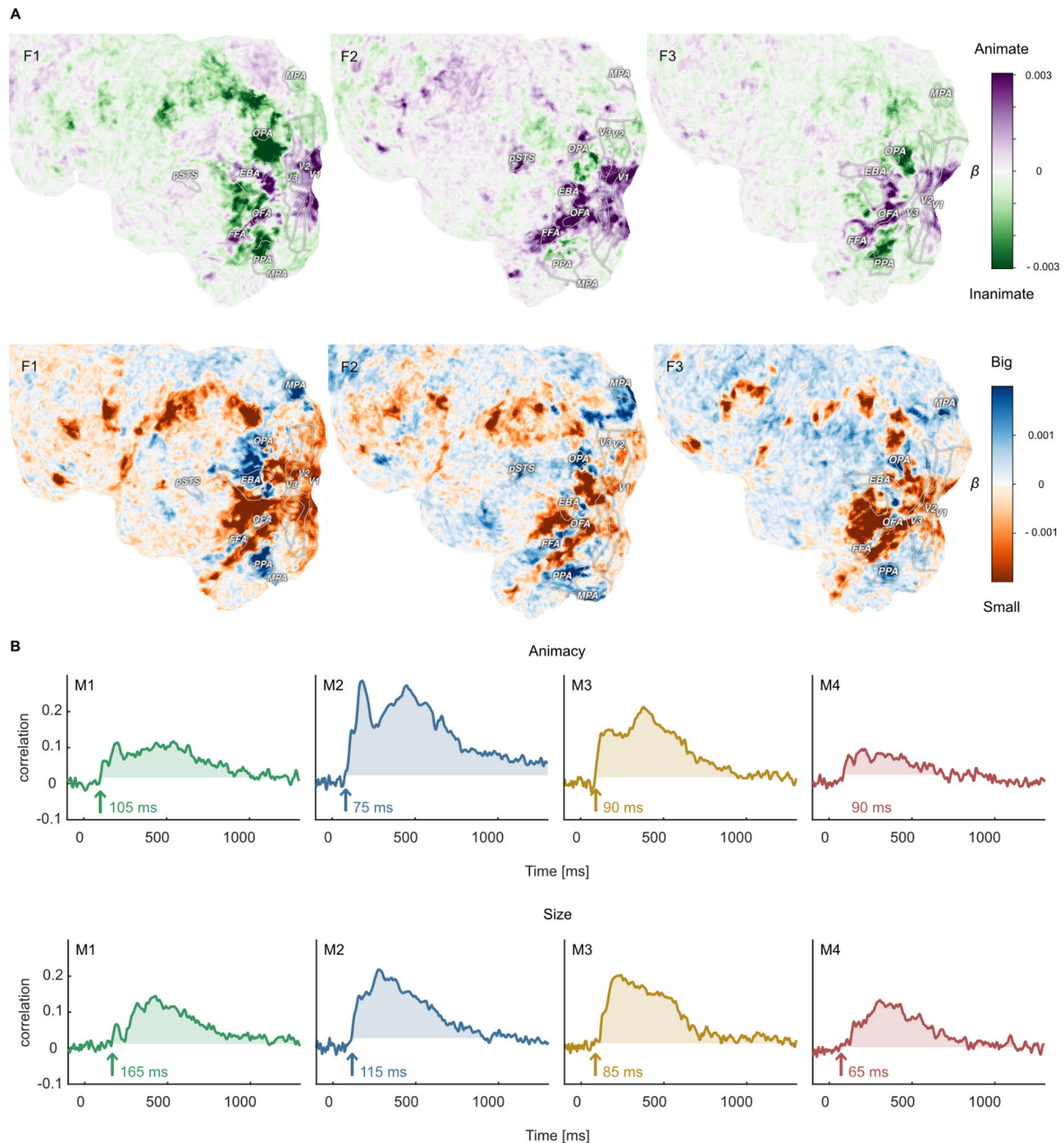
Fig. 6. Functional topography and temporal dynamics of object animacy and size. A. Voxel-wise regression weights for object animacy and size as predictors of trial-wise fMRI responses. The results replicate the characteristic spoke-like topography of functional tuning to animacy and size in occipitotemporal cortex. B. Time courses for the animacy (top) and size (bottom) information in the MEG signal. The time courses were obtained from a cross-validated linear regression and show the correlation between the predicted and true animacy and size labels. Shaded areas reflect the largest time window exceeding the maximum correlation during the baseline period.
