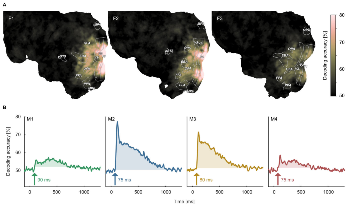
Fig. 4. Object image decoding in fMRI and MEG. A. Decoding accuracies in the fMRI data from a searchlight-based pairwise classification analysis visualized on the cortical surface. B. Analogous decoding accuracies in the MEG data plotted over time. The arrow marks the onset of the largest time window where accuracies exceeded the threshold which was defined as the maximum decoding accuracy observed during the baseline period.
